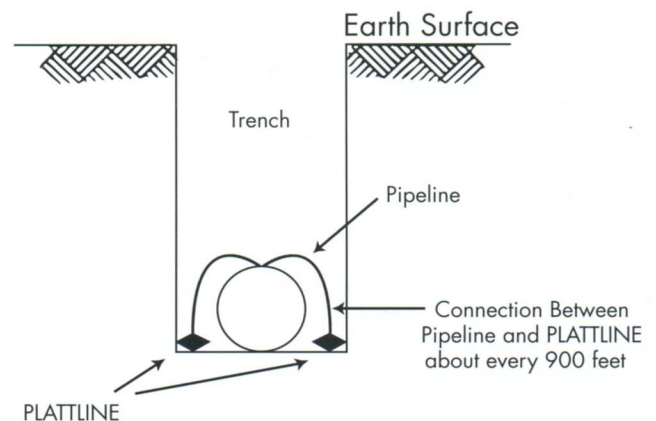
Figure 2 - Plattline connections to the pipe
