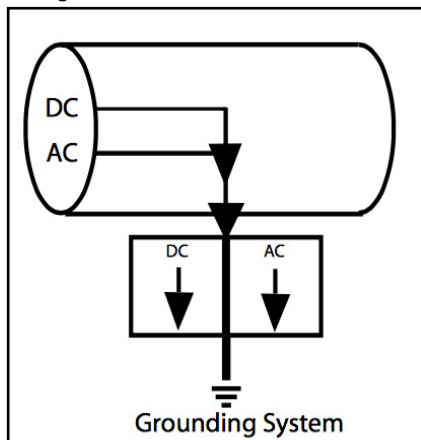
FIGURE 2 "Short Circuit" Mode For Over-Voltage Protection
