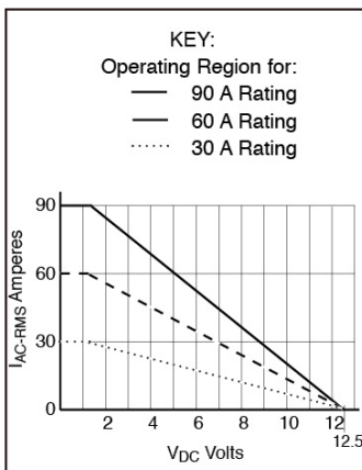
FIGURE 3 Maximum Steady-State 60 Hz AC Current vs. DC Voltage For B Code = 12.5
