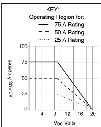
FIGURE 6 Maximum Steady-State 50 Hz AC Current vs. DC Voltage For B Code = 20
