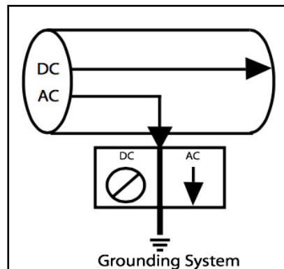
FIGURE 1 The ISP in Normal Mode For Cathodic Isolation
