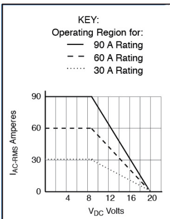
FIGURE 4 Maximum Steady-State 60 Hz AC Current vs. DC Voltage For B Code = 20
